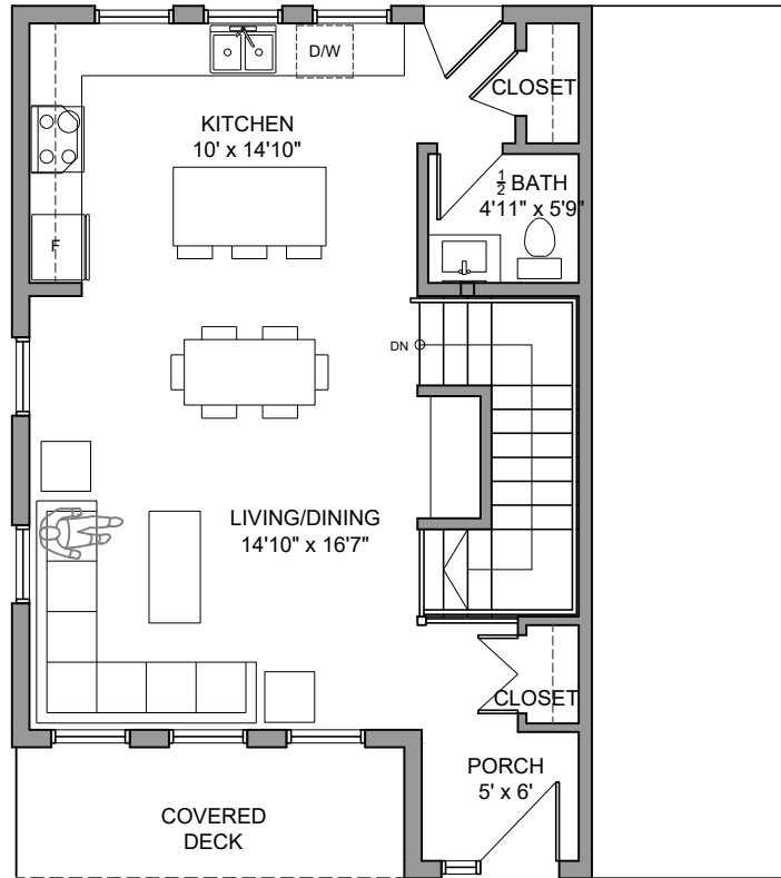
GRADE LEVEL
